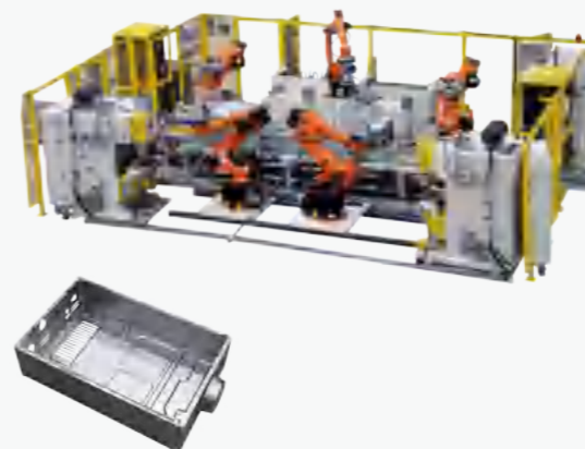
燃气热水器底盖组焊一体化全自动生产线 Automatic Welder For Shell And Base Plate
