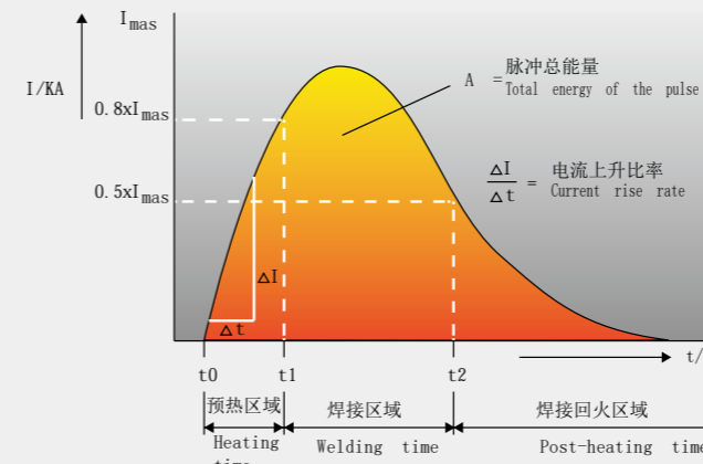
电容储能放电曲线 Capacitor Energy Storage Discharge Curve
