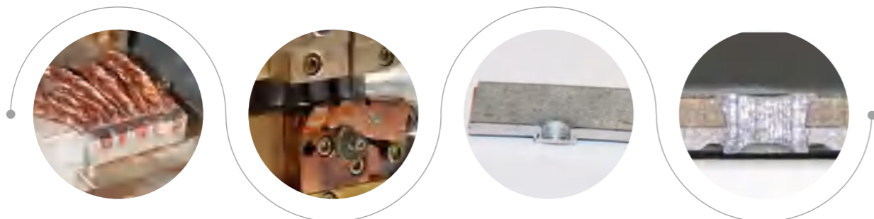
电阻扩散焊 Resistance Diffusion Welding 电阻钎焊 Resistance Brazing 无铆钉铆接 Tog-L-Loc 平面自冲铆 Flush Self-Piercing Riveting
